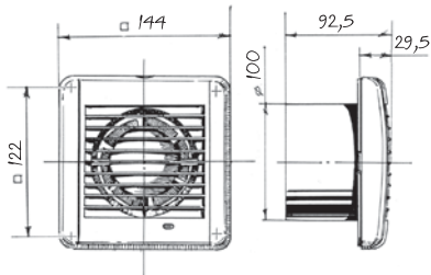
Square grille
