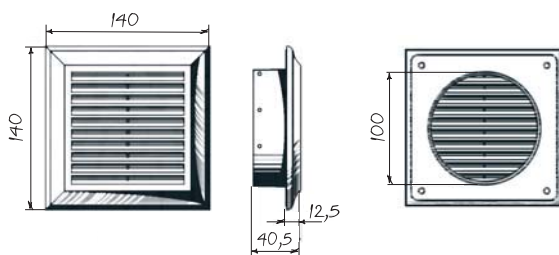
Square grille
